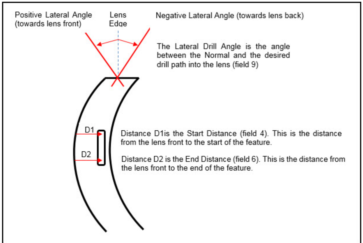
FIGURE 7: SIDE DRILLING START DISTANCE, END DISTANCE, AND LATERAL ANGLE VIEWED FROM THE LENS SIDE
