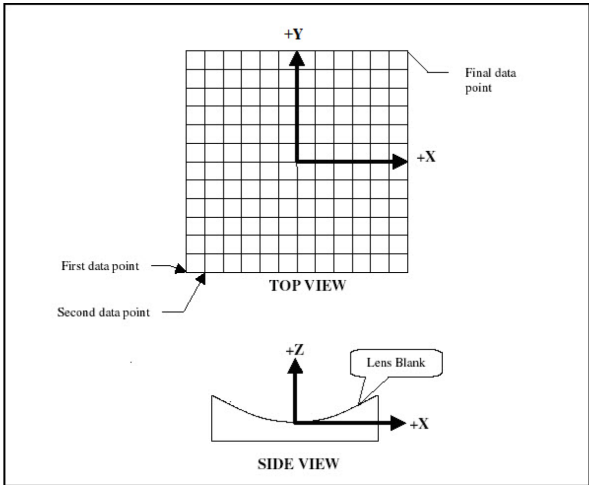
FIGURE 10: SURFACE MATRIX ORIENTATION
