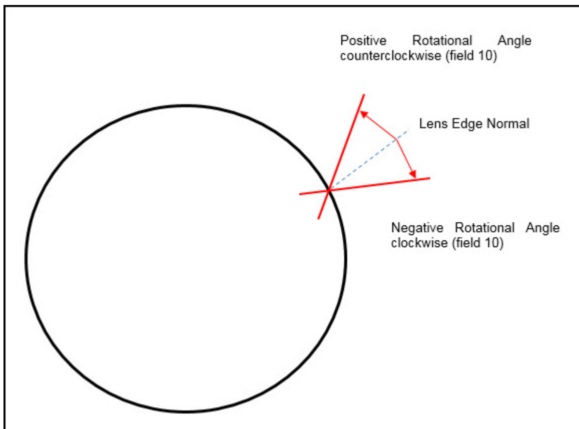
FIGURE 8: SIDE DRILLING ROTATIONAL ANGLE VIEWED FORM THE LENS FRONT
