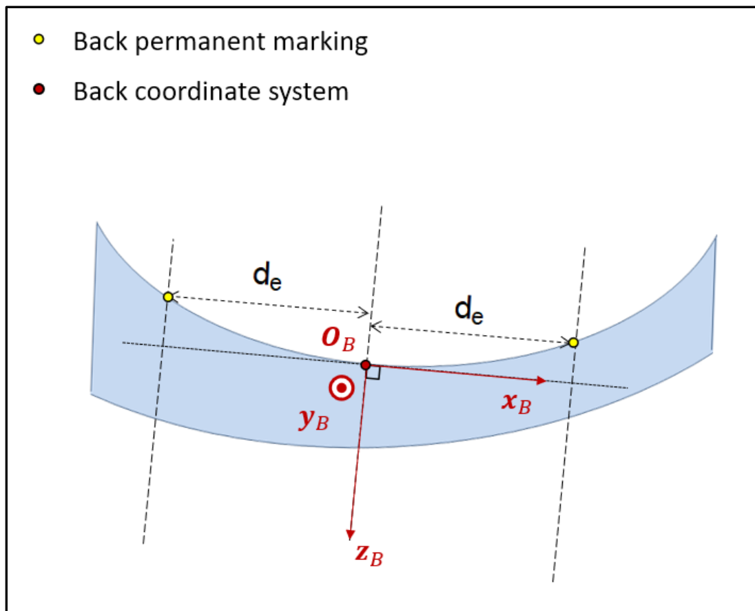
FIGURE 2: BACK ENGRAVINGS REFERENCE COORDINATE SYSTEM
