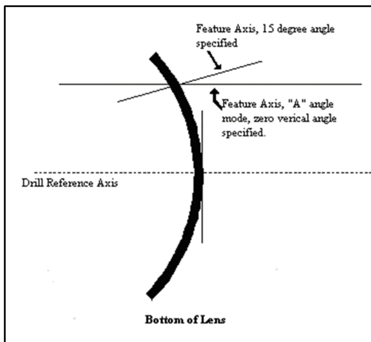
FIGURE 5: VERTICAL ANGLE
