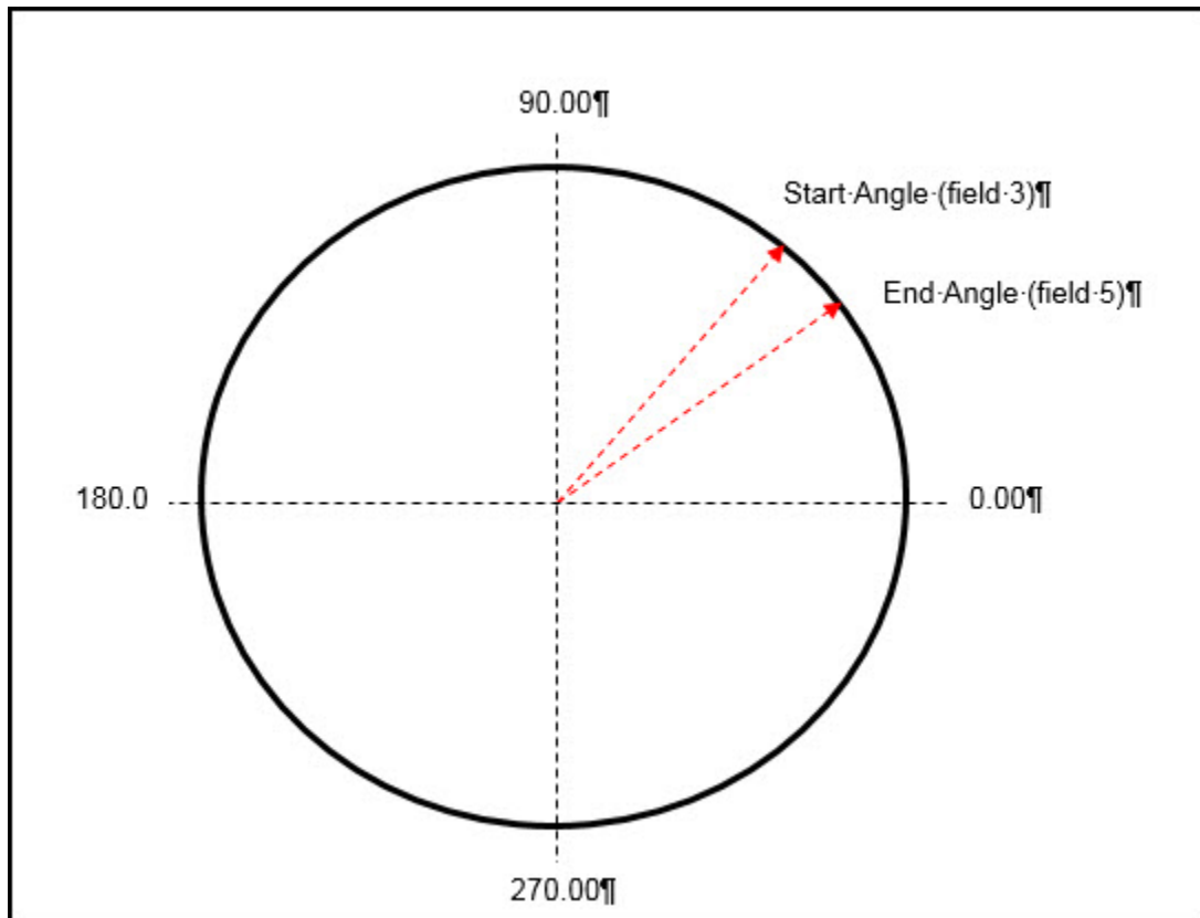
FIGURE 6: LOCATION OF A SIDE DRILLING FEATURE (START ANGLE, END ANGLE) VIEWED FROM THE LENS FRONT
