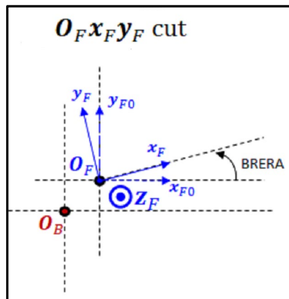
FIGURE 4: TRANSFER FROM THE LENS REFERENCE COORDINATE SYSTEM ON THE BACK ( O_B x_B y_B z_B ) TO THE REFERENCE COORDINATE SYSTEM ON THE FRONT ( O_F x_F y_F z_F )
