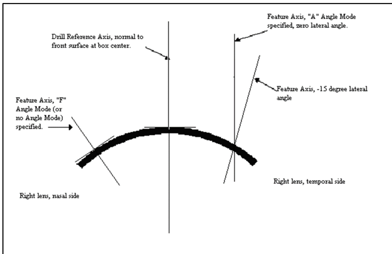
FIGURE 4: LATERAL ANGLE
