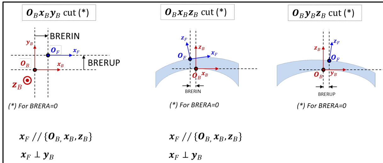
FIGURE 3: DEFINITION OF THE LENS REFERENCE COORDINATE SYSTEM ON THE FRONT ( O_F x_F y_F z_F ) ACCORDING TO THE REFERENCE COORDINATE SYSTEM ON THE BACK ( O_B x_B y_B z_B )
